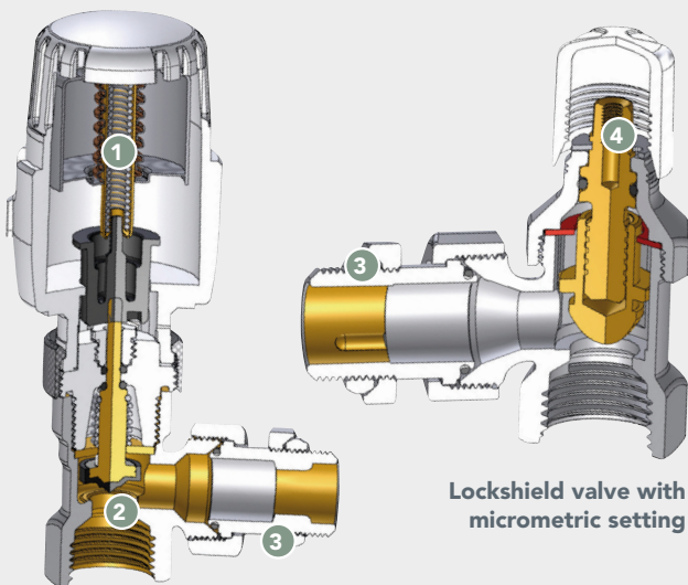
Thermostatic valve
